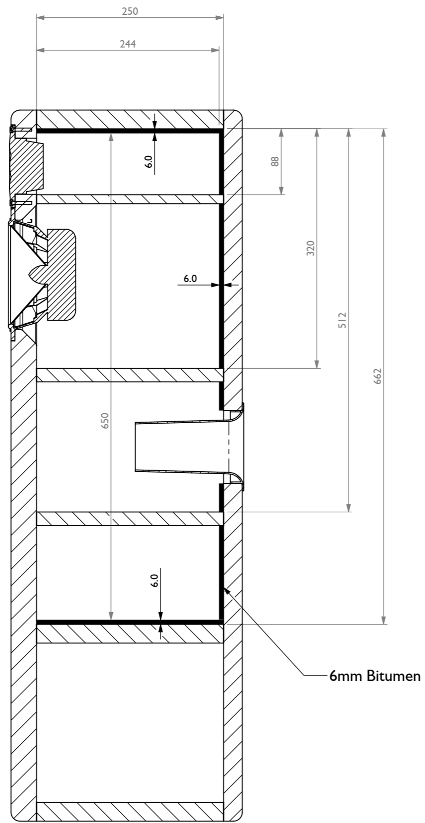
SECTION X-X
